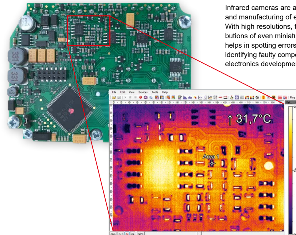
Microscope optics can be used to detect smallest details. The temperature is measured on an area of 16 x 10 mm.
