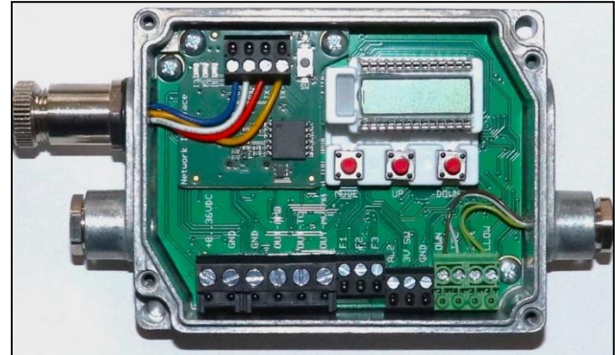
Installation of the Network Interface board into Optris CT Electronic Box
