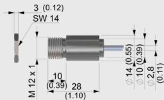
Sensing head
